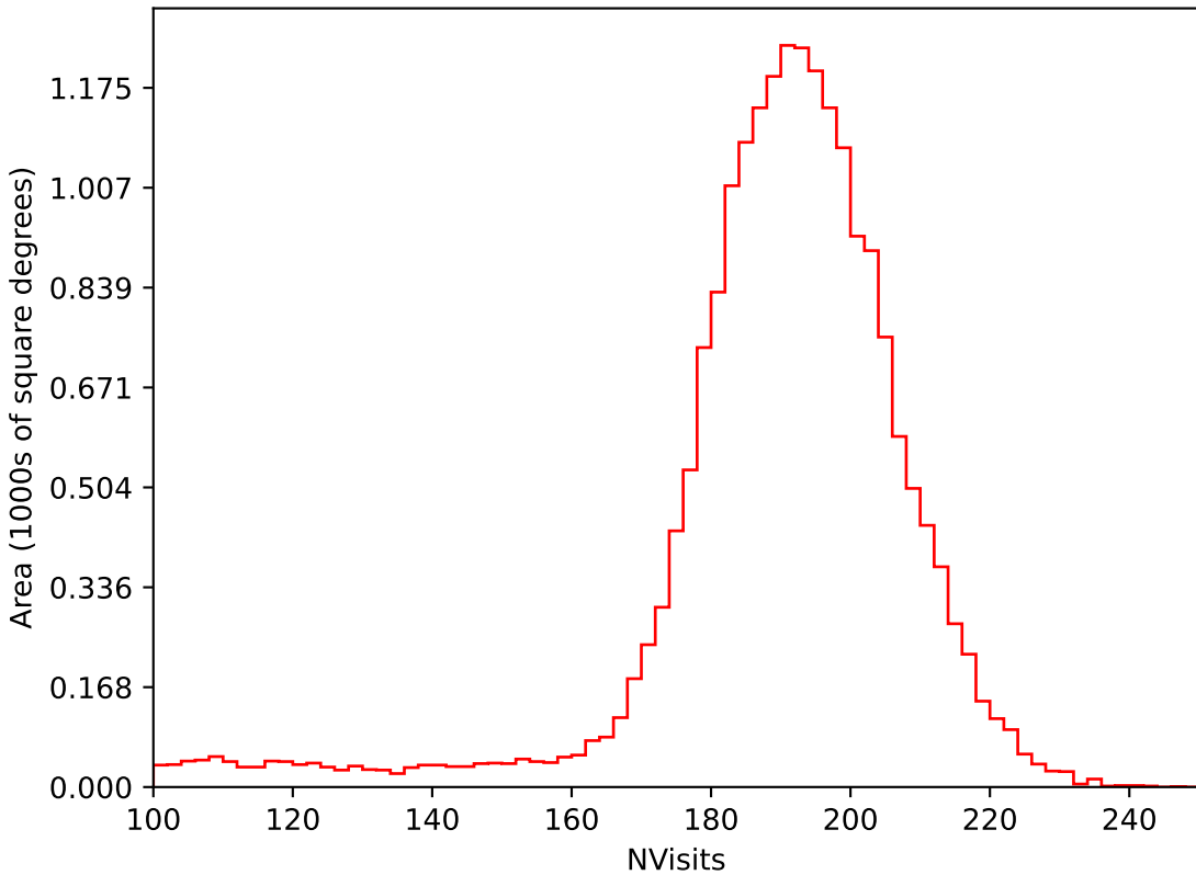
too_10_4v3.4_10yrs All sky i band: NVisits
