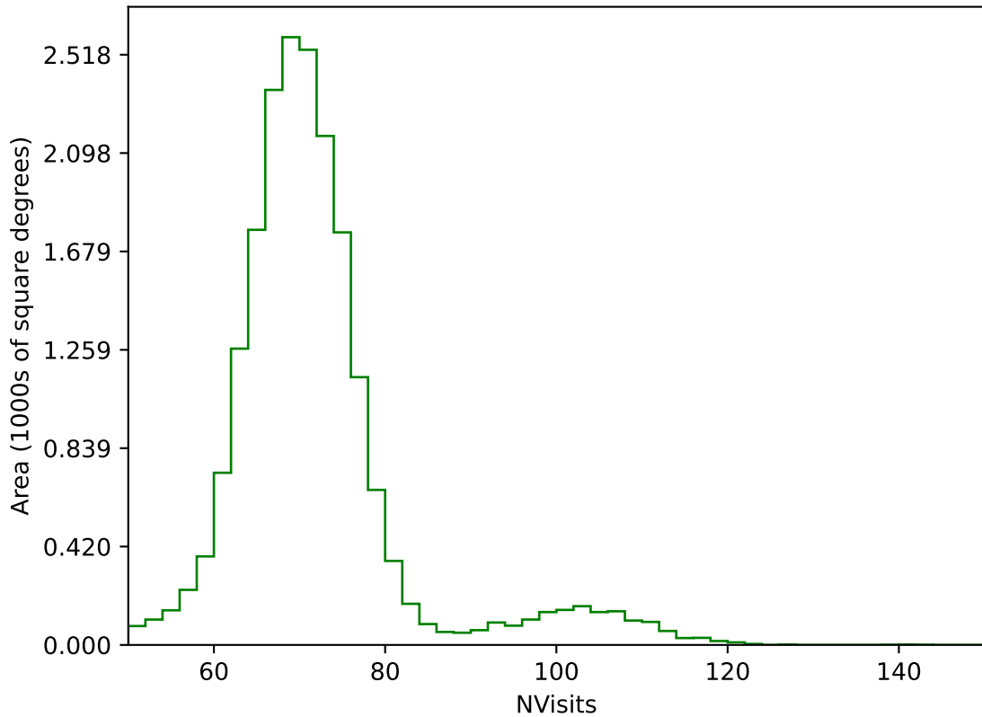
too_10_4v3.4_10yrs All sky g band: NVisits
