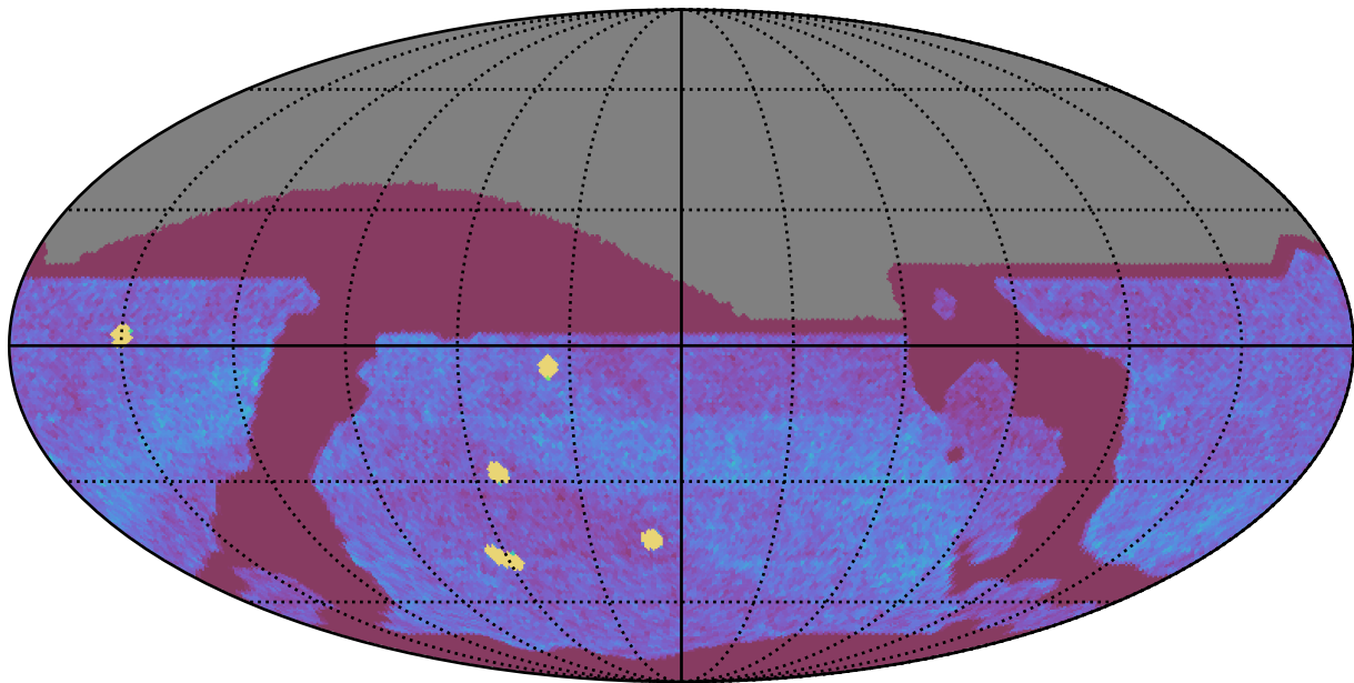
too_10_4v3.4_10yrs All sky all bands: NVisits
