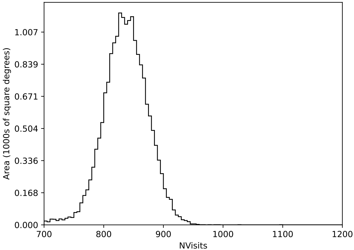
too_10_4v3.4_10yrs All sky all bands: NVisits
