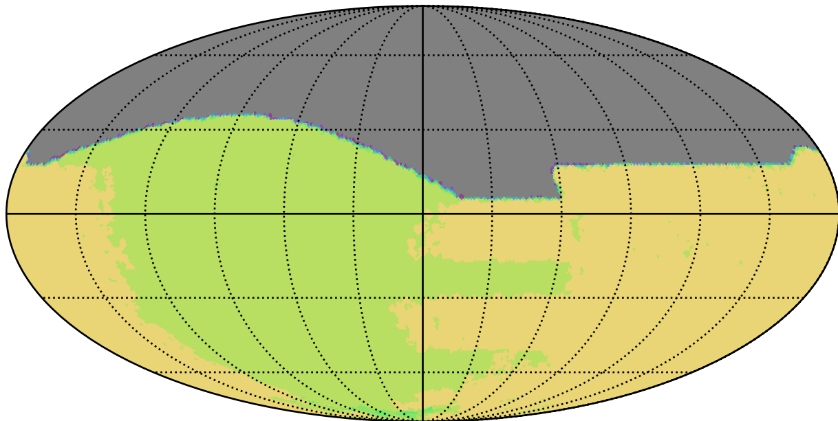
too_10_4v3.4_10yrs All sky all bands: NSeasons
