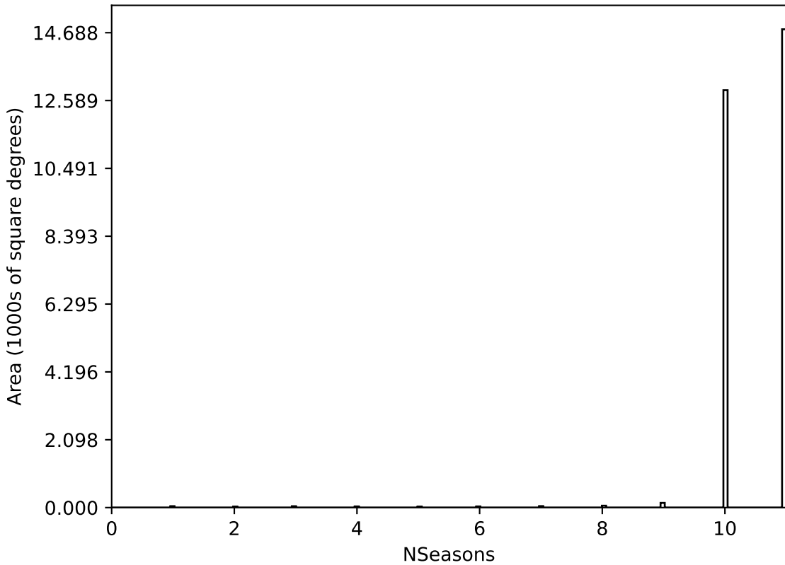
too_10_4v3.4_10yrs All sky all bands: NSeasons
