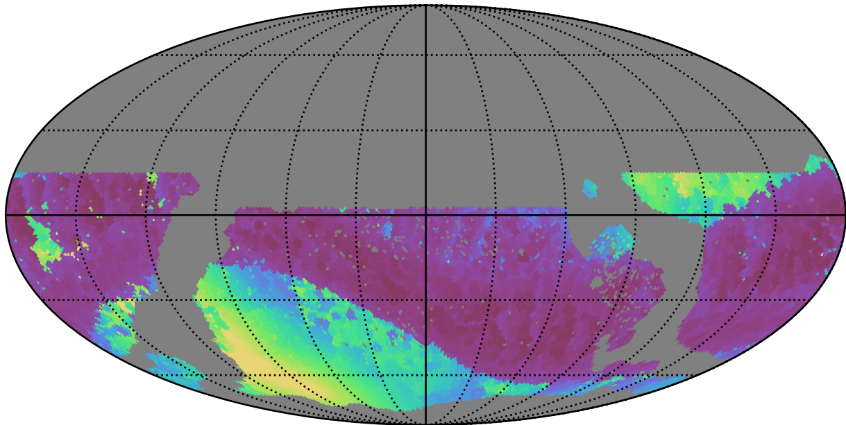
too_10_4v3.4_10yrs WFD z band: Min solarElong
