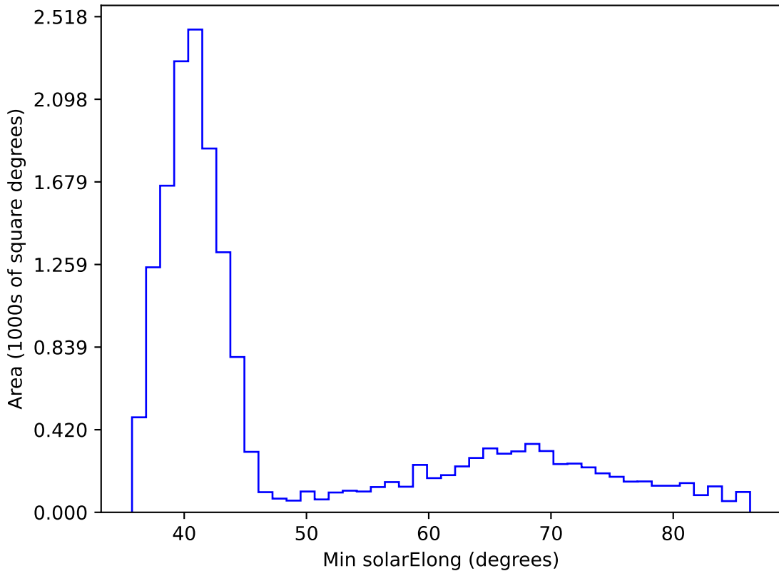
too_10_4v3.4_10yrs WFD z band: Min solarElong
