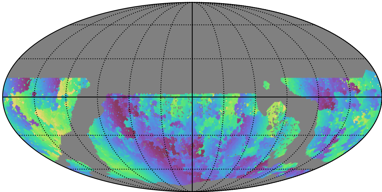
too_10_4v3.4_10yrs WFD u band: Min solarElong
