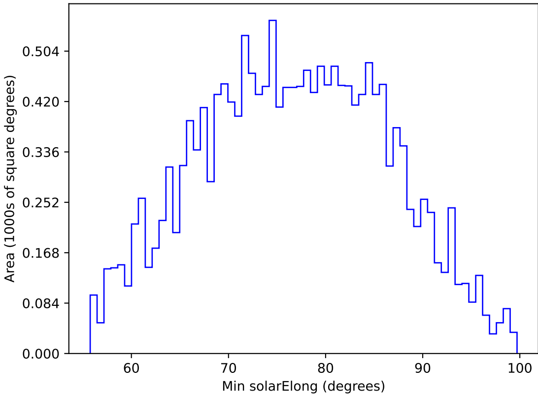
too_10_4v3.4_10yrs WFD u band: Min solarElong
