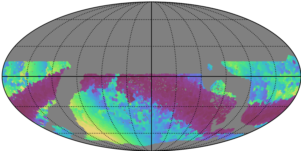
too_10_4v3.4_10yrs WFD r band: Min solarElong
