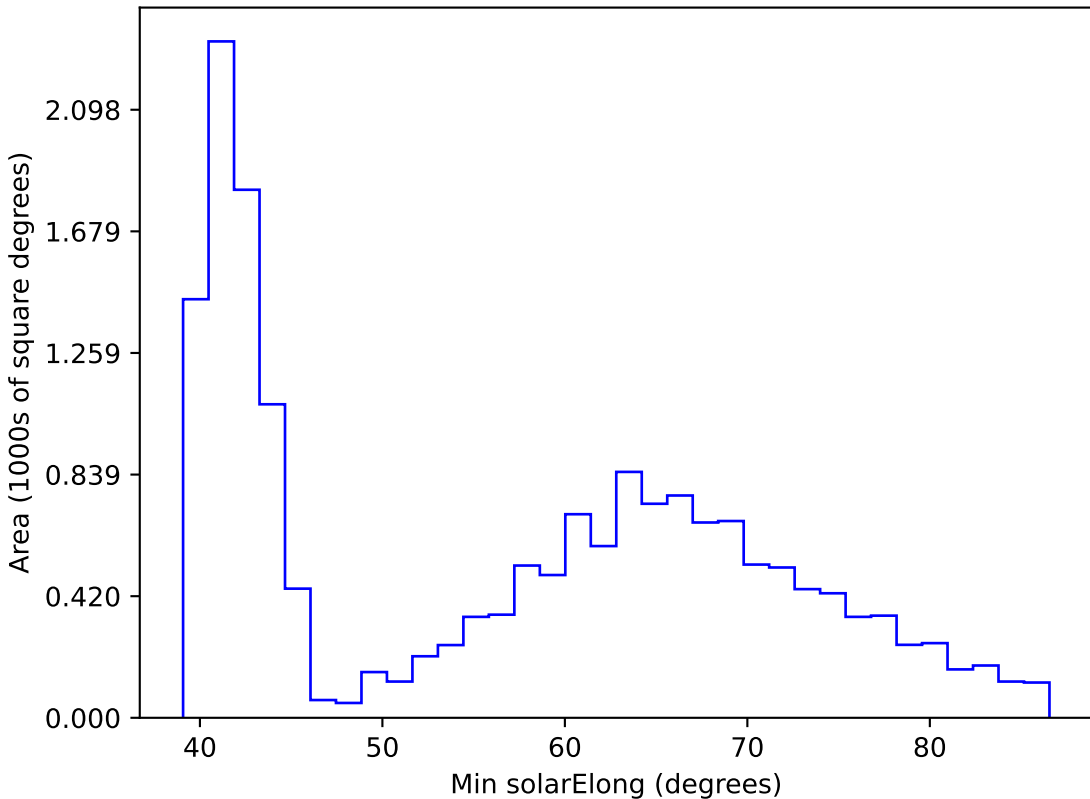
too_10_4v3.4_10yrs WFD r band: Min solarElong
