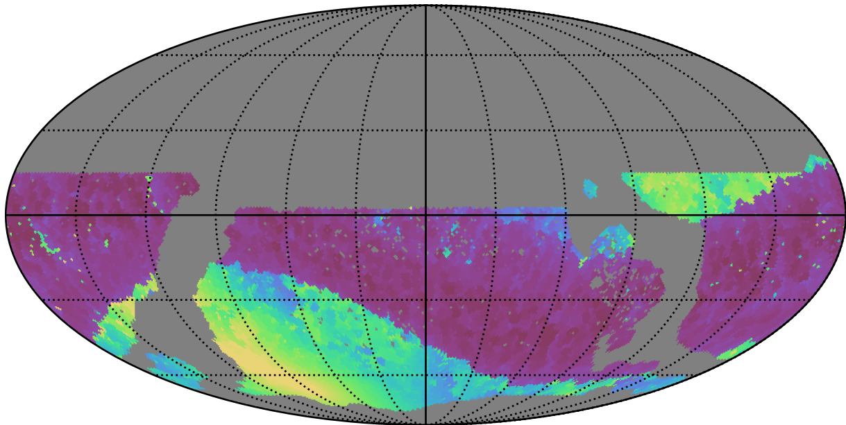
too_10_4v3.4_10yrs WFD i band: Min solarElong
