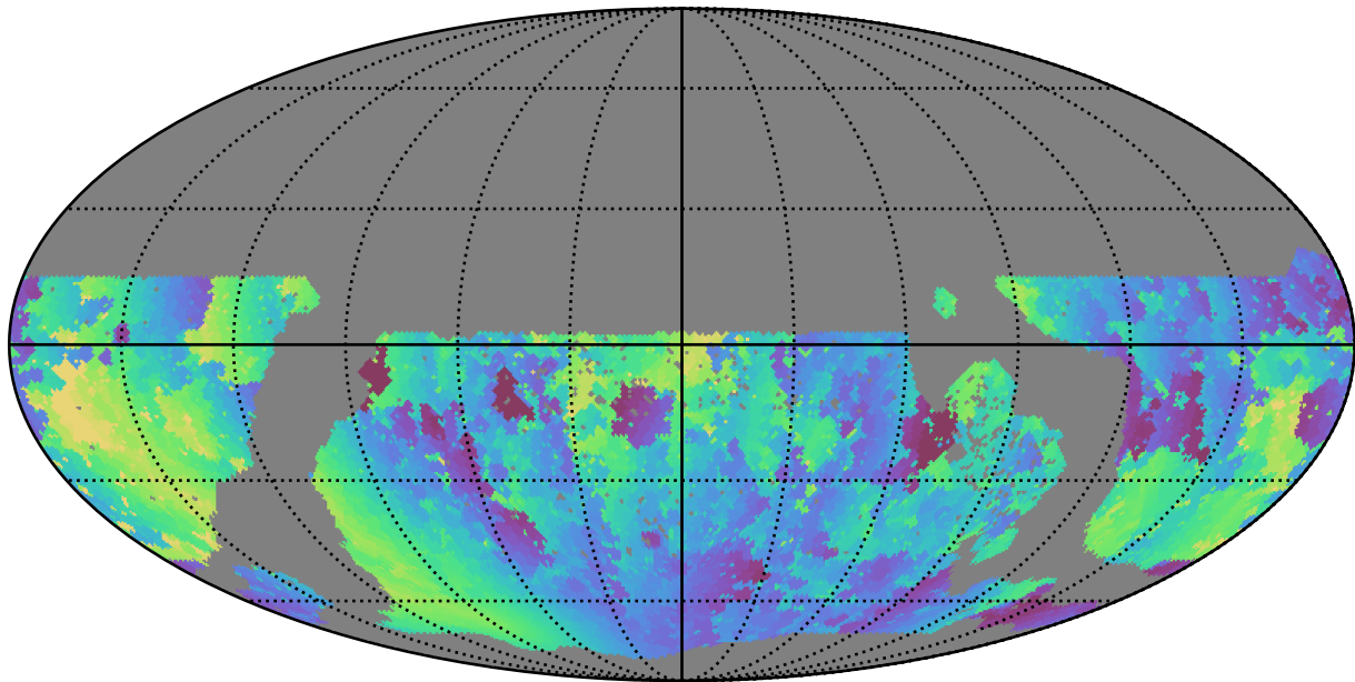
too_10_4v3.4_10yrs WFD g band: Min solarElong
