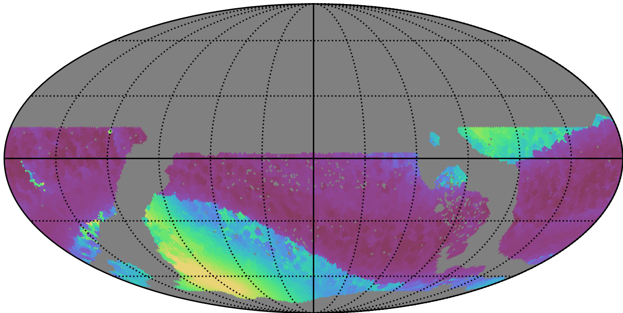
too_10_4v3.4_10yrs WFD all bands: Min solarElong
