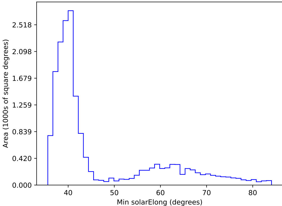
too_10_4v3.4_10yrs WFD all bands: Min solarElong
