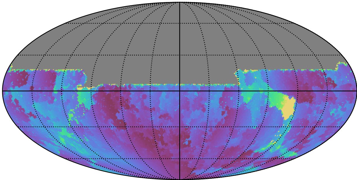
too_10_4v3.4_10yrs All sky u band: Min solarElong
