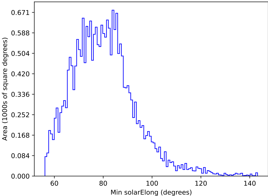
too_10_4v3.4_10yrs All sky u band: Min solarElong
