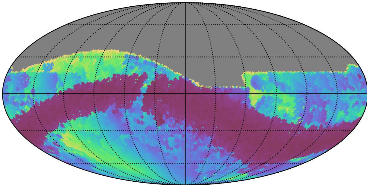
too_10_4v3.4_10yrs All sky r band: Min solarElong
