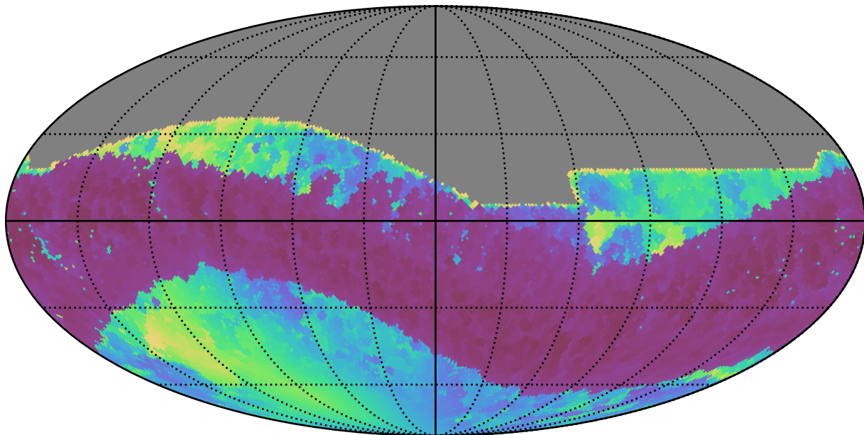
too_10_4v3.4_10yrs All sky i band: Min solarElong
