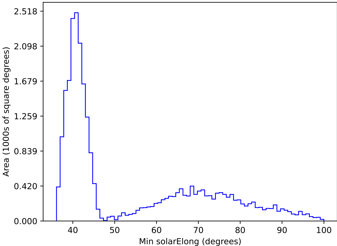
too_10_4v3.4_10yrs All sky i band: Min solarElong
