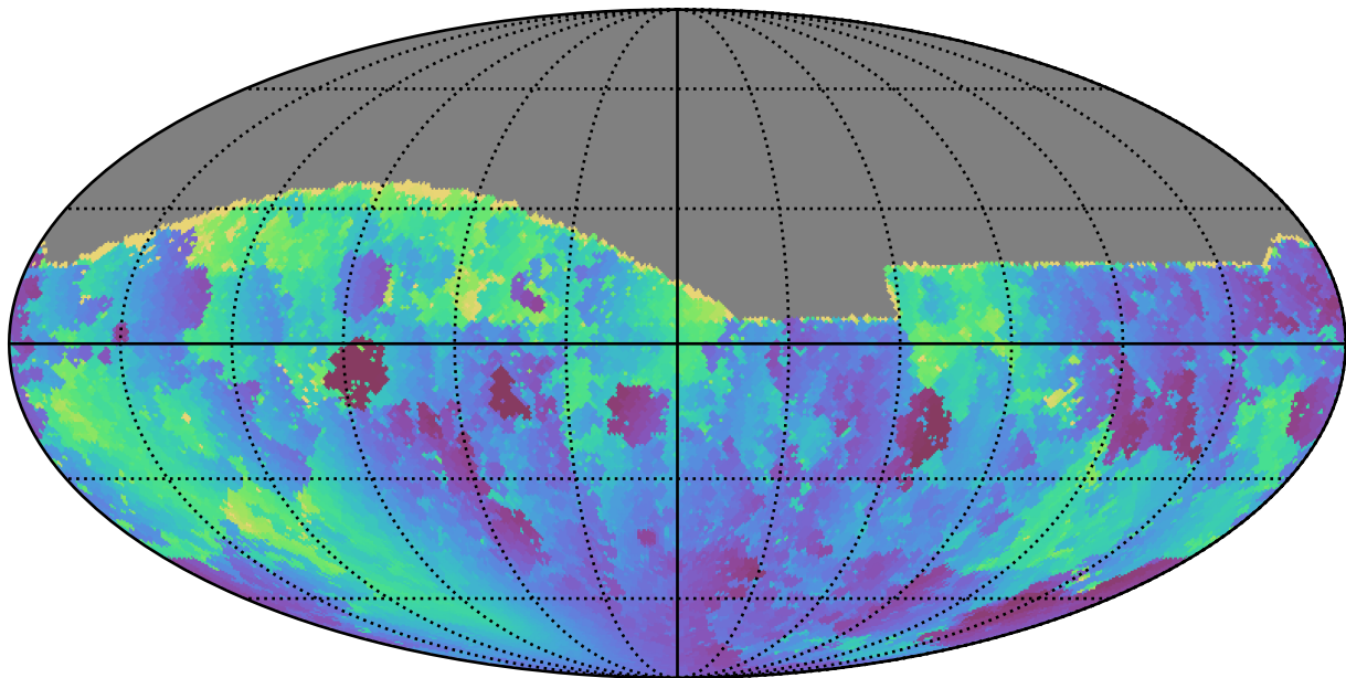
too_10_4v3.4_10yrs All sky g band: Min solarElong
