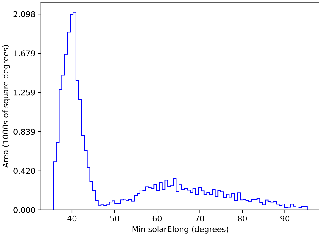
too_10_4v3.4_10yrs All sky all bands: Min solarElong
