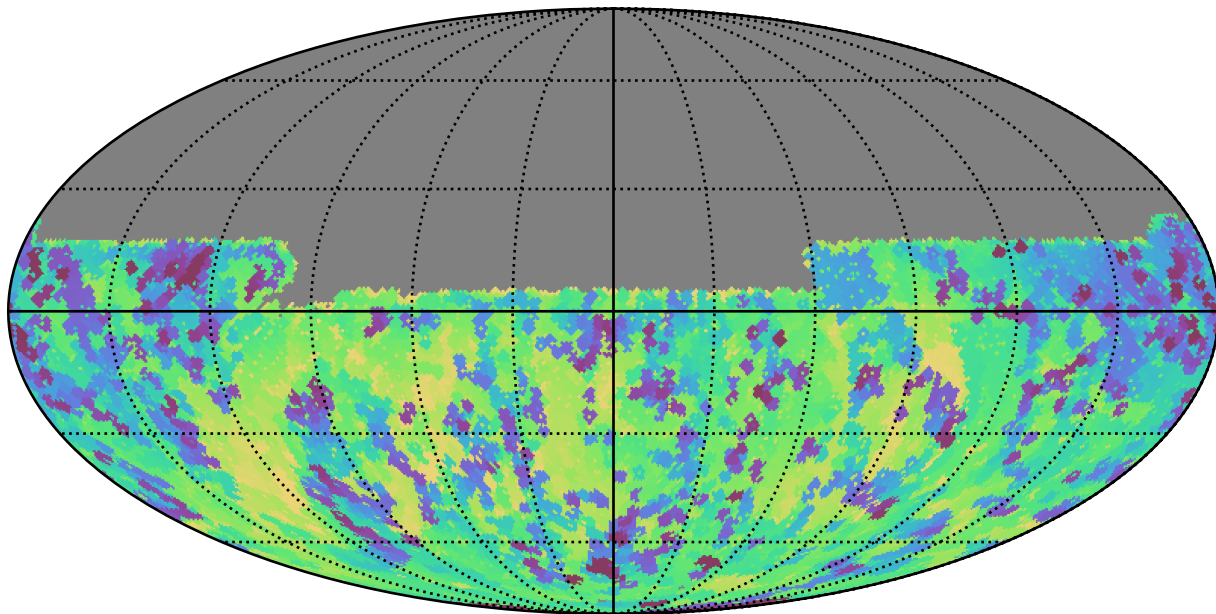
too_10_4v3.4_10yrs Yr 1 y band: Min skyBrightness
