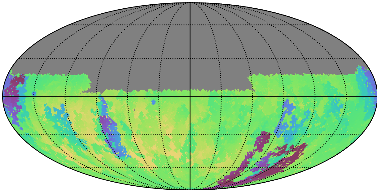
too_10_4v3.4_10yrs Yr 1 u band: Min skyBrightness
