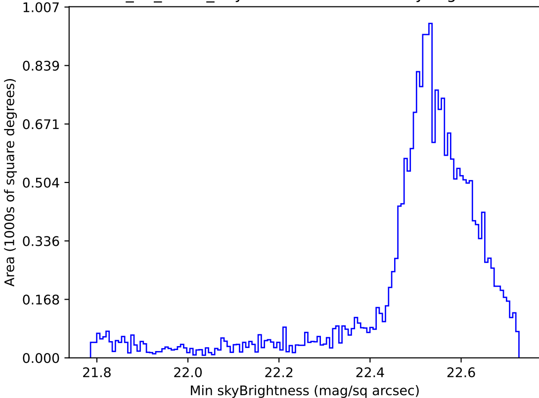
too_10_4v3.4_10yrs Yr 1 u band: Min skyBrightness
