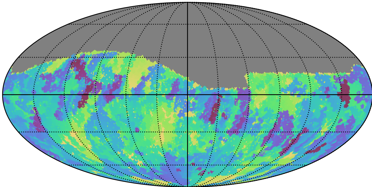
too_10_4v3.4_10yrs Yr 1 r band: Min skyBrightness
