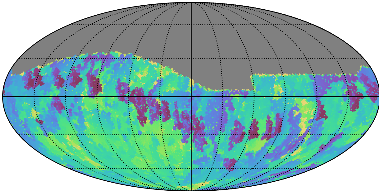
too_10_4v3.4_10yrs Yr 1 i band: Min skyBrightness
