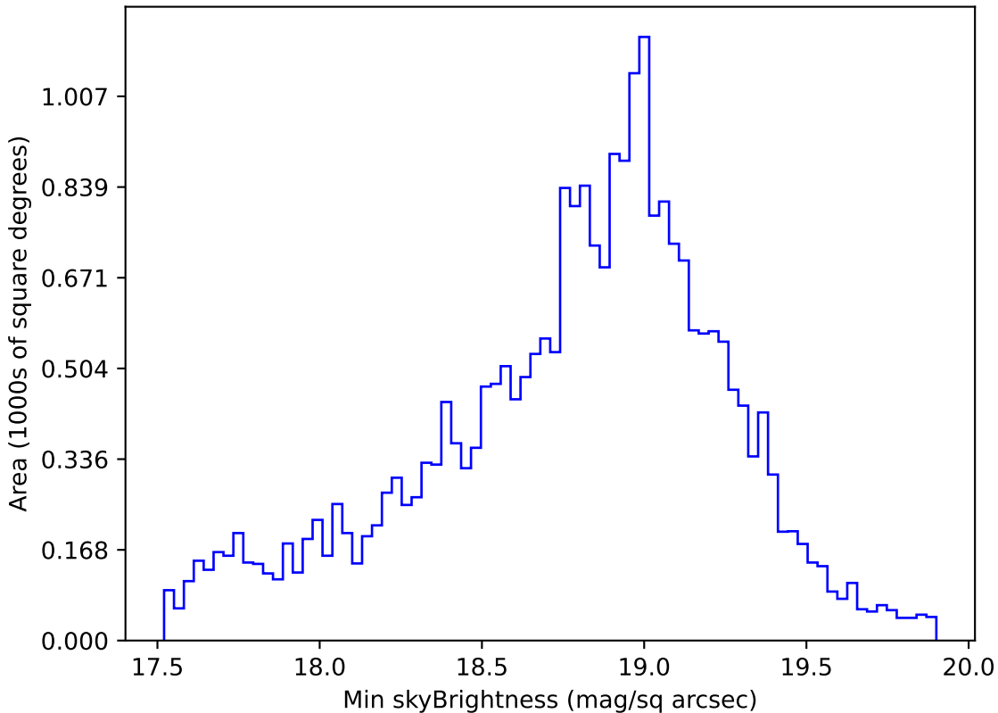
too_10_4v3.4_10yrs Yr 1 i band: Min skyBrightness
