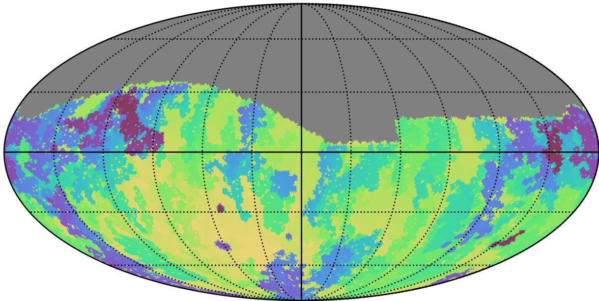
too_10_4v3.4_10yrs Yr 1 g band: Min skyBrightness
