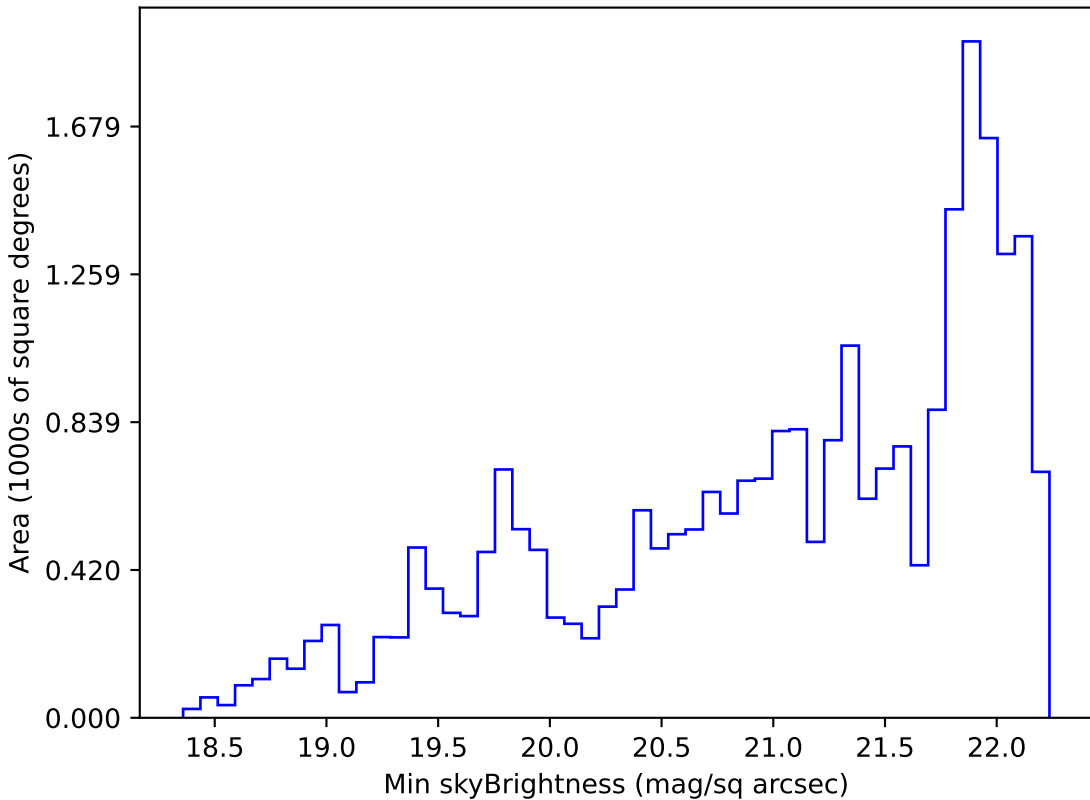
too_10_4v3.4_10yrs Yr 1 g band: Min skyBrightness
