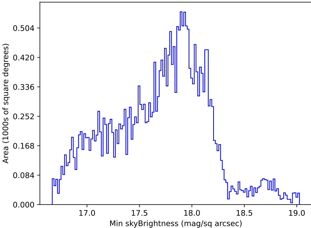
too_10_4v3.4_10yrs Yr 1 all bands: Min skyBrightness
