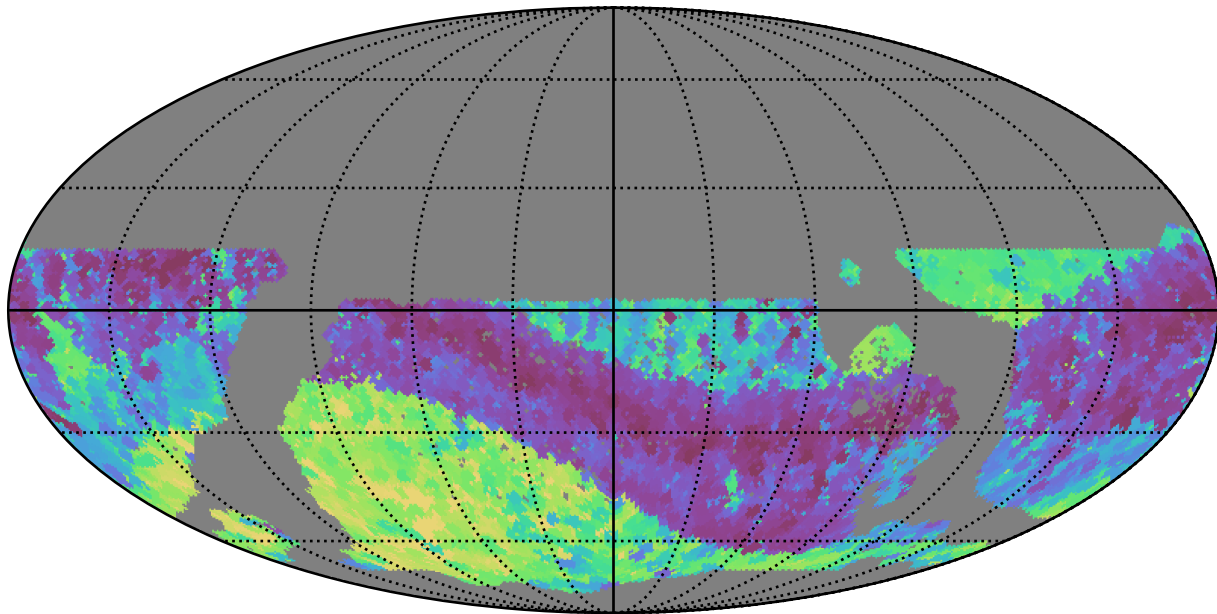
too_10_4v3.4_10yrs WFD z band: Min skyBrightness
