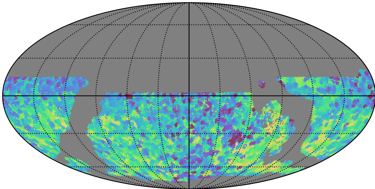
too_10_4v3.4_10yrs WFD y band: Min skyBrightness
