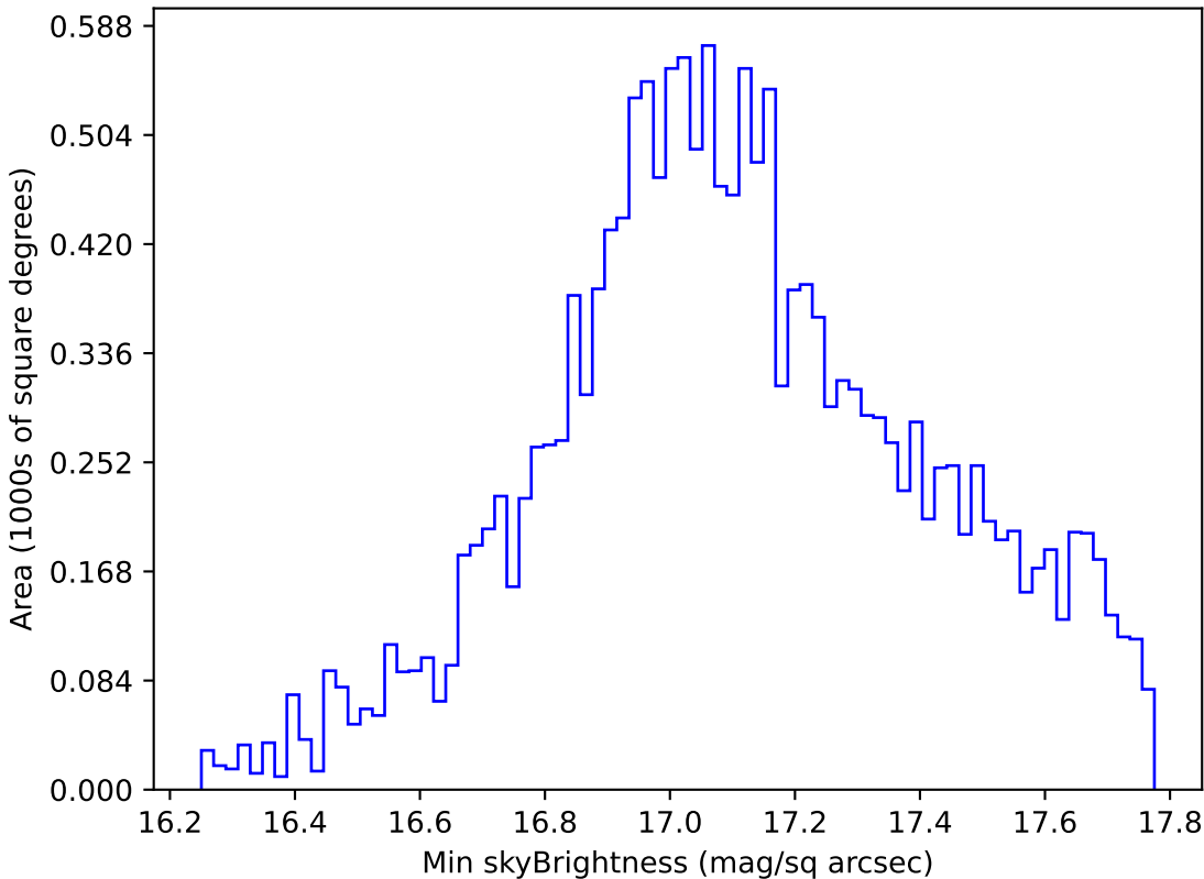
too_10_4v3.4_10yrs WFD y band: Min skyBrightness
