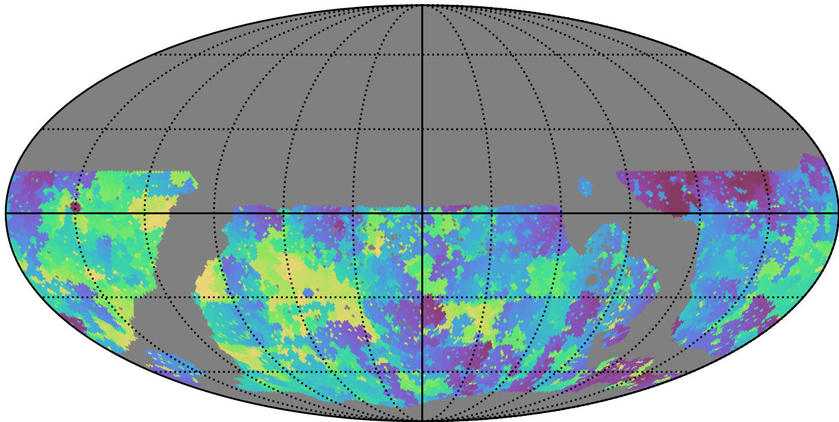
too_10_4v3.4_10yrs WFD u band: Min skyBrightness
