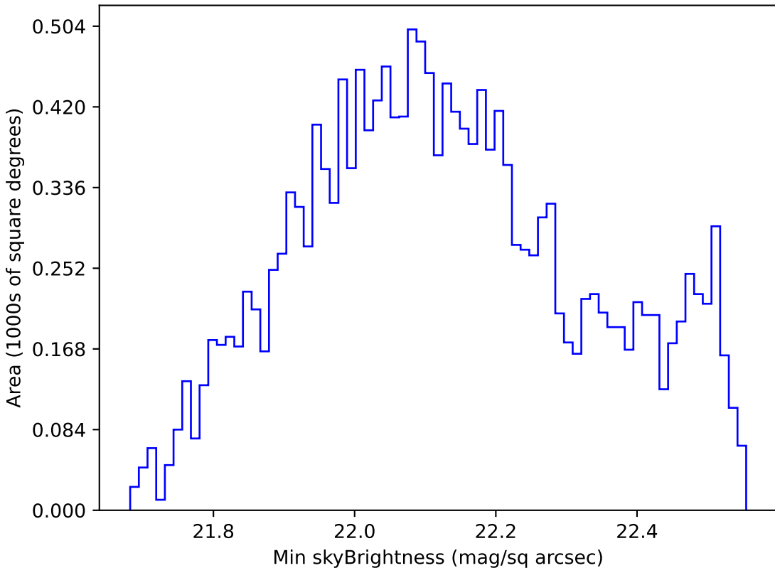
too_10_4v3.4_10yrs WFD u band: Min skyBrightness
