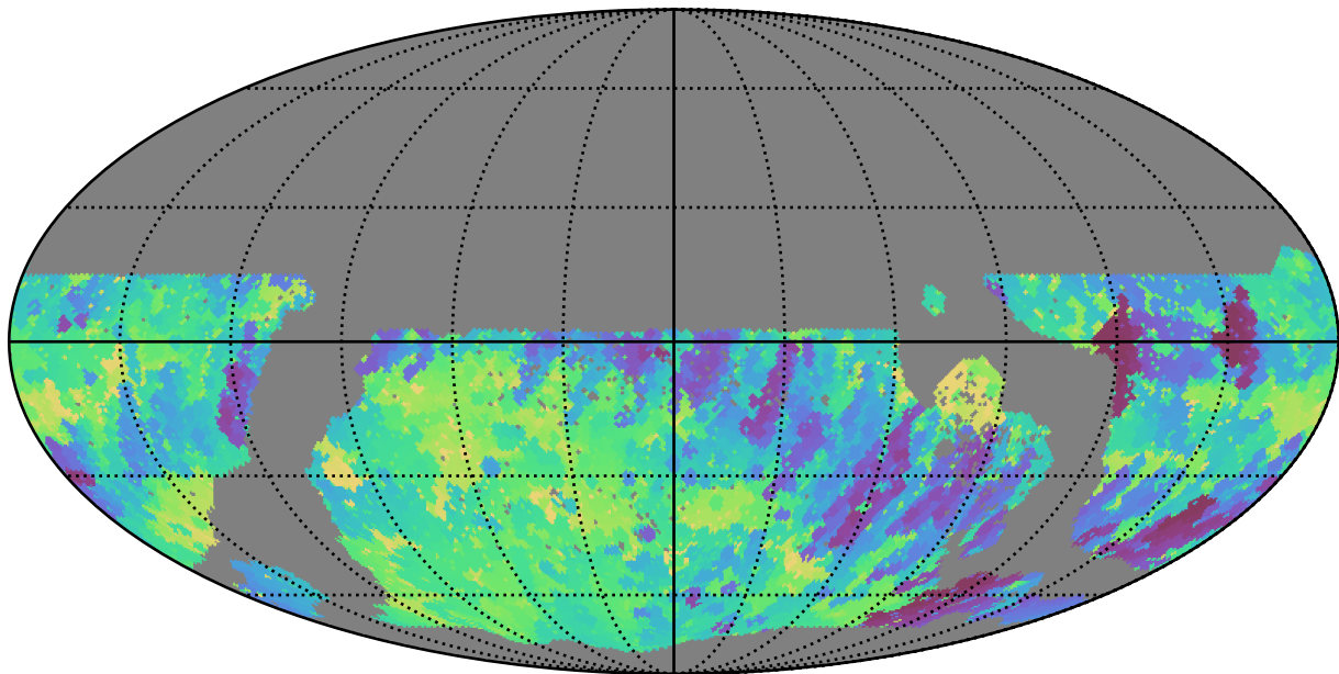
too_10_4v3.4_10yrs WFD r band: Min skyBrightness
