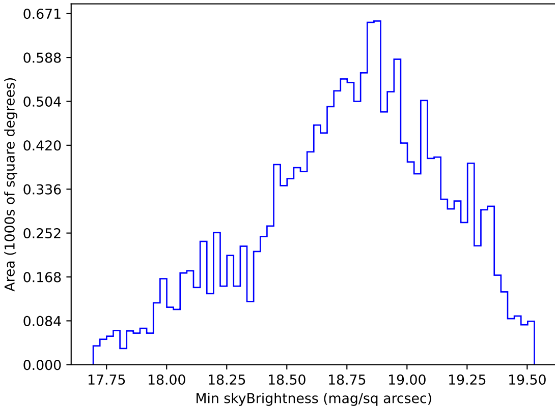
too_10_4v3.4_10yrs WFD r band: Min skyBrightness
