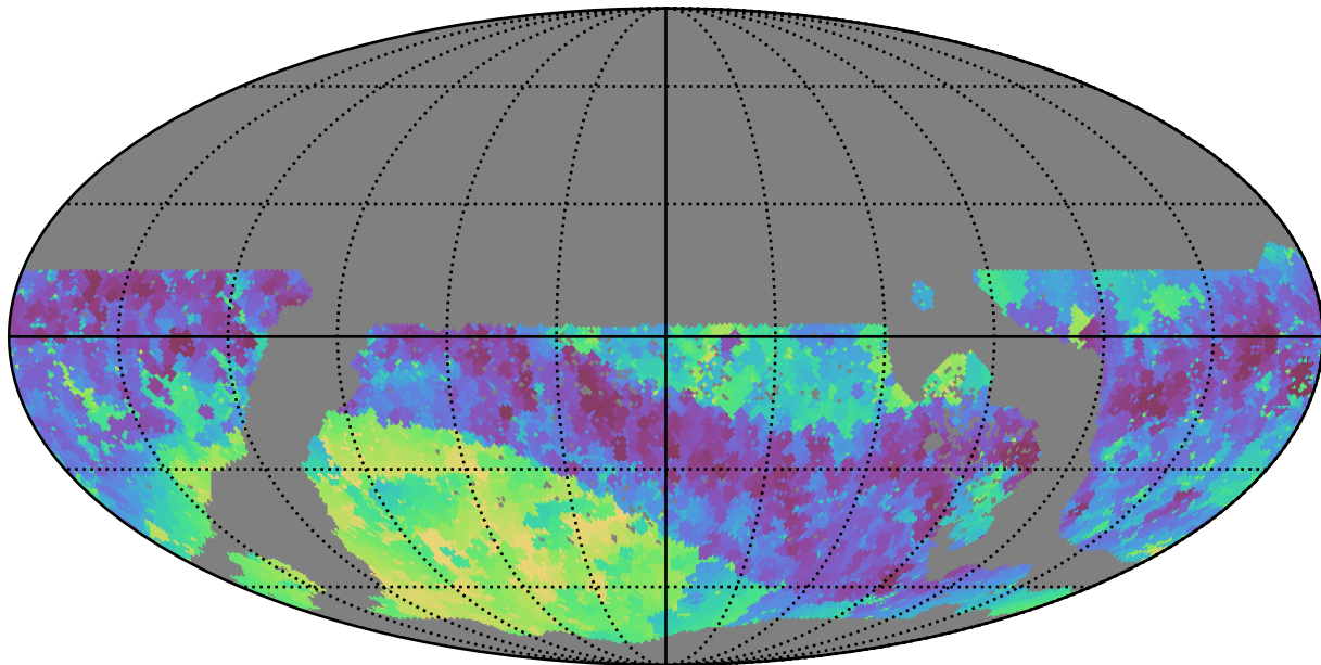
too_10_4v3.4_10yrs WFD i band: Min skyBrightness
