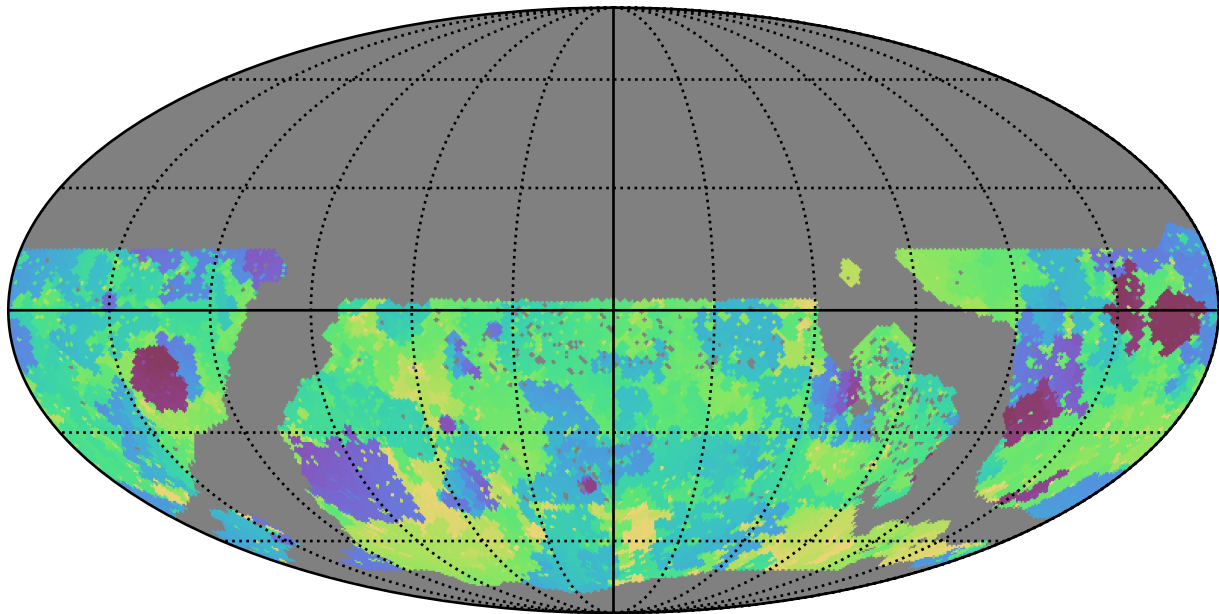
too_10_4v3.4_10yrs WFD g band: Min skyBrightness
