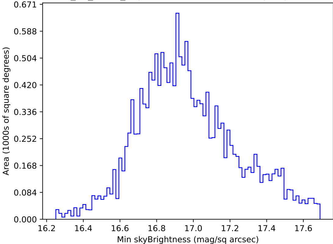
too_10_4v3.4_10yrs WFD all bands: Min skyBrightness
