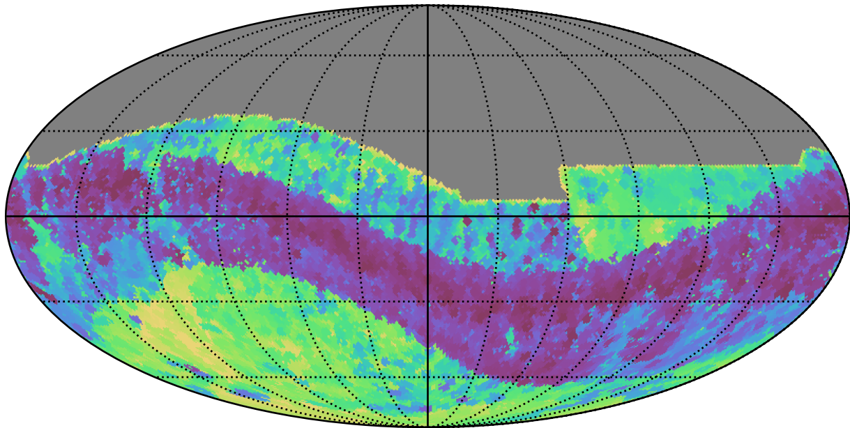
too_10_4v3.4_10yrs All sky z band: Min skyBrightness
