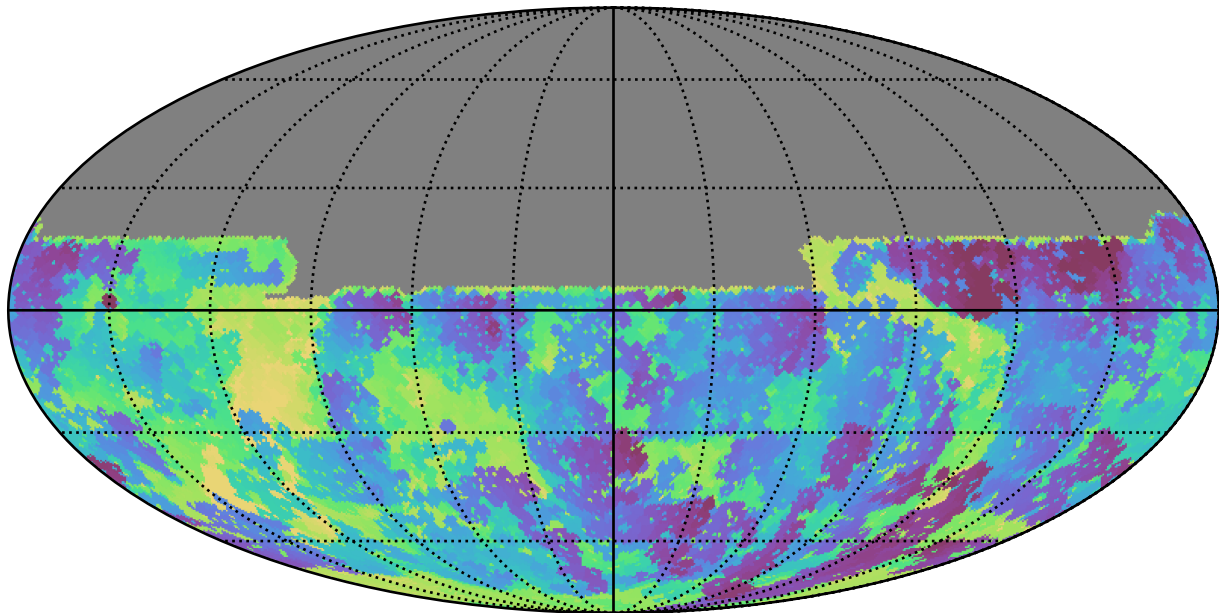
too_10_4v3.4_10yrs All sky u band: Min skyBrightness
