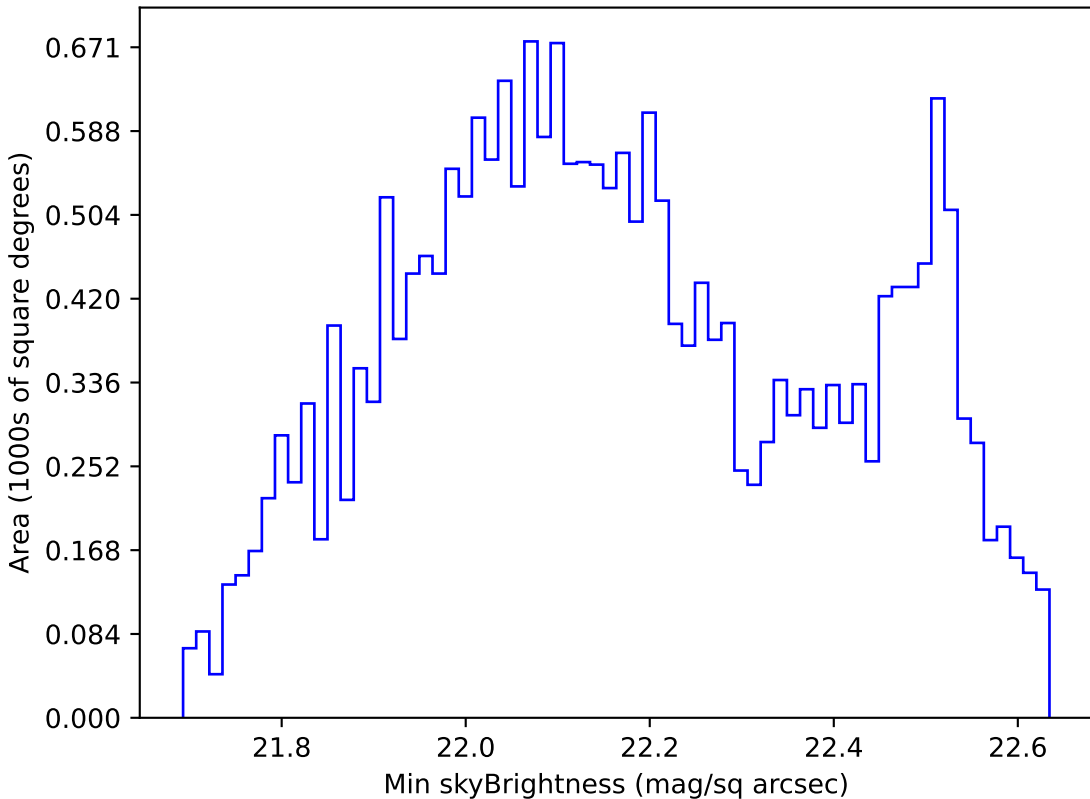
too_10_4v3.4_10yrs All sky u band: Min skyBrightness
