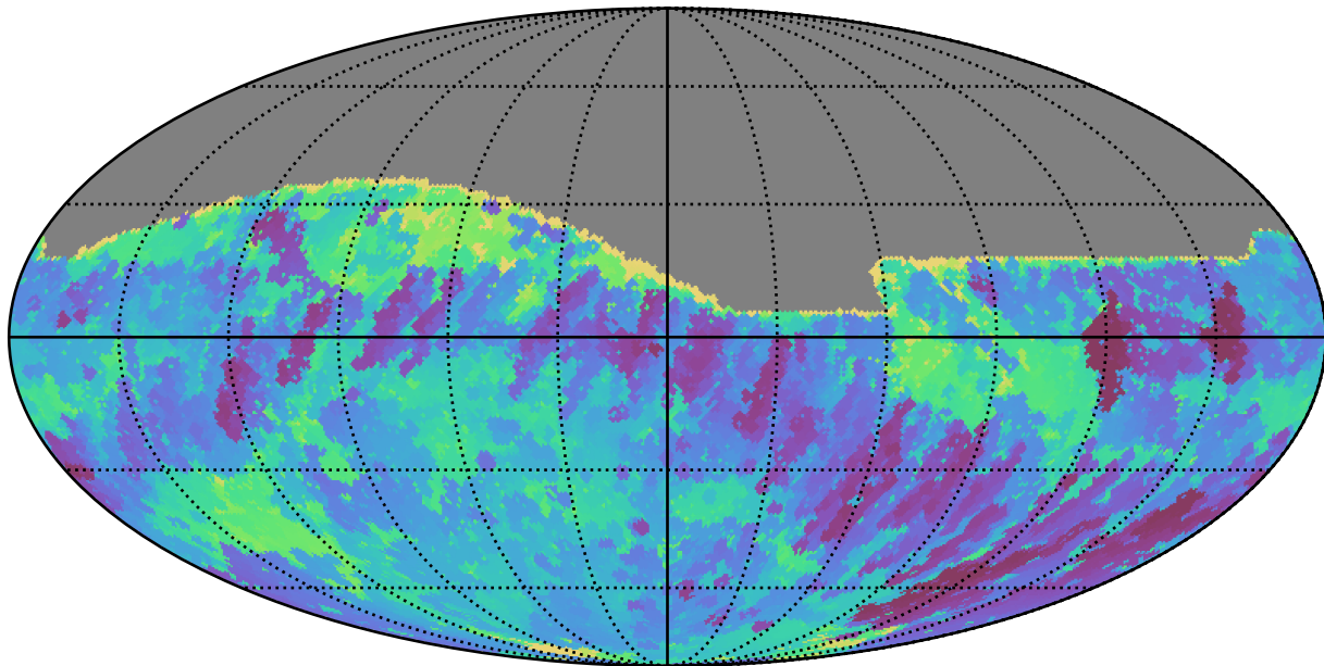
too_10_4v3.4_10yrs All sky r band: Min skyBrightness
