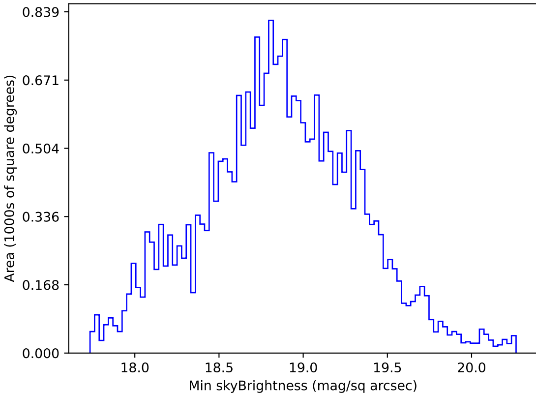
too_10_4v3.4_10yrs All sky r band: Min skyBrightness
