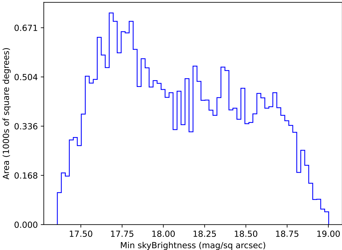
too_10_4v3.4_10yrs All sky i band: Min skyBrightness
