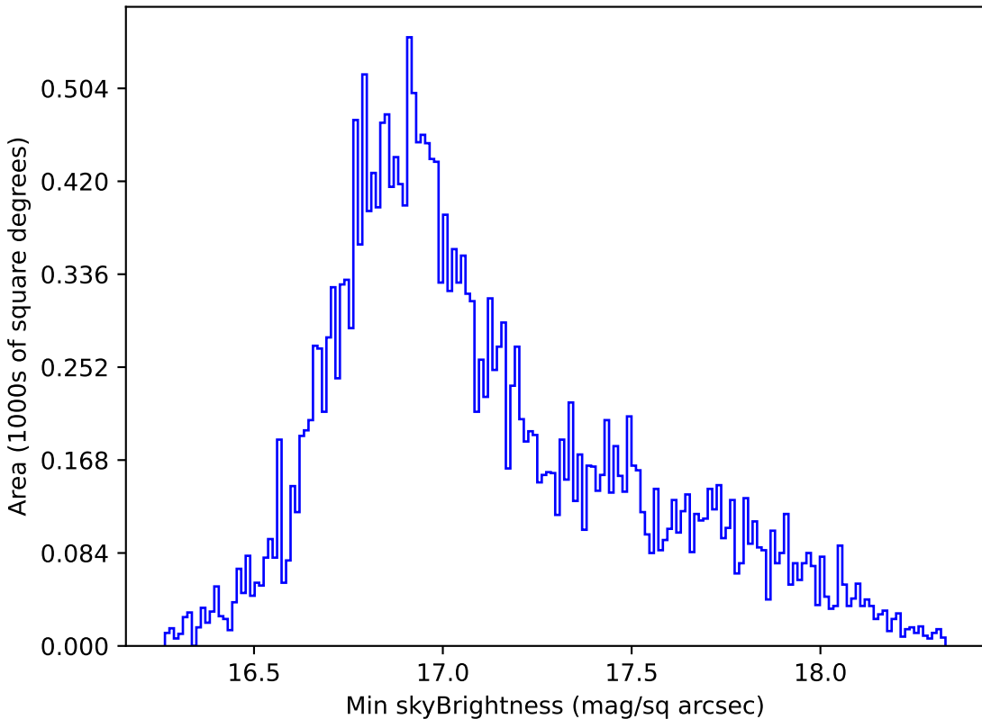
too_10_4v3.4_10yrs All sky all bands: Min skyBrightness
