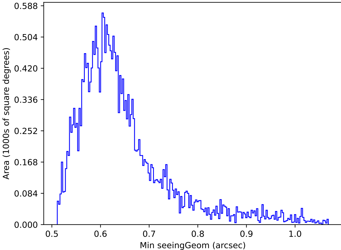
too_10_4v3.4_10yrs Yr 1 z band: Min seeingGeom
